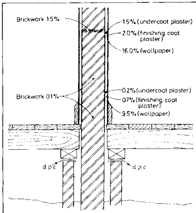
Concentration of salts in a party wall in which rising damp has persisted for 80 years. The figures show the percentage by weight of chloride plus nitrate. The shaded area is heavily contaminated. (Redrawn from Building Research Establishment Digest 245, revised 1987)
